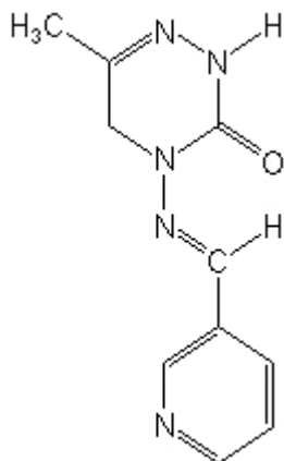
Figure 3.2.118-1 Chemical structure of pymetrozine
